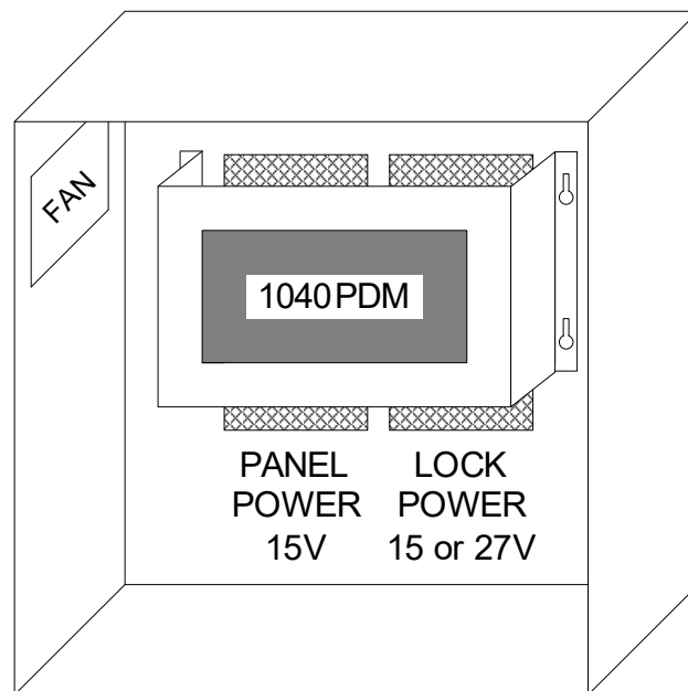
Figure 2 1040PE Enclosure
