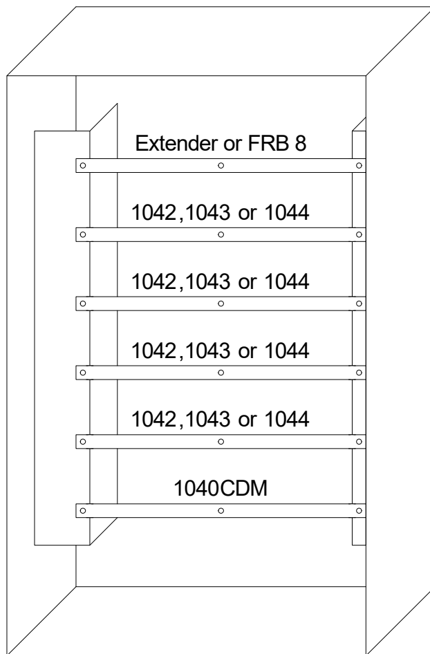
Figure 1 1040E Enclosure
